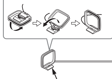
AM loop antenna (supplied)
